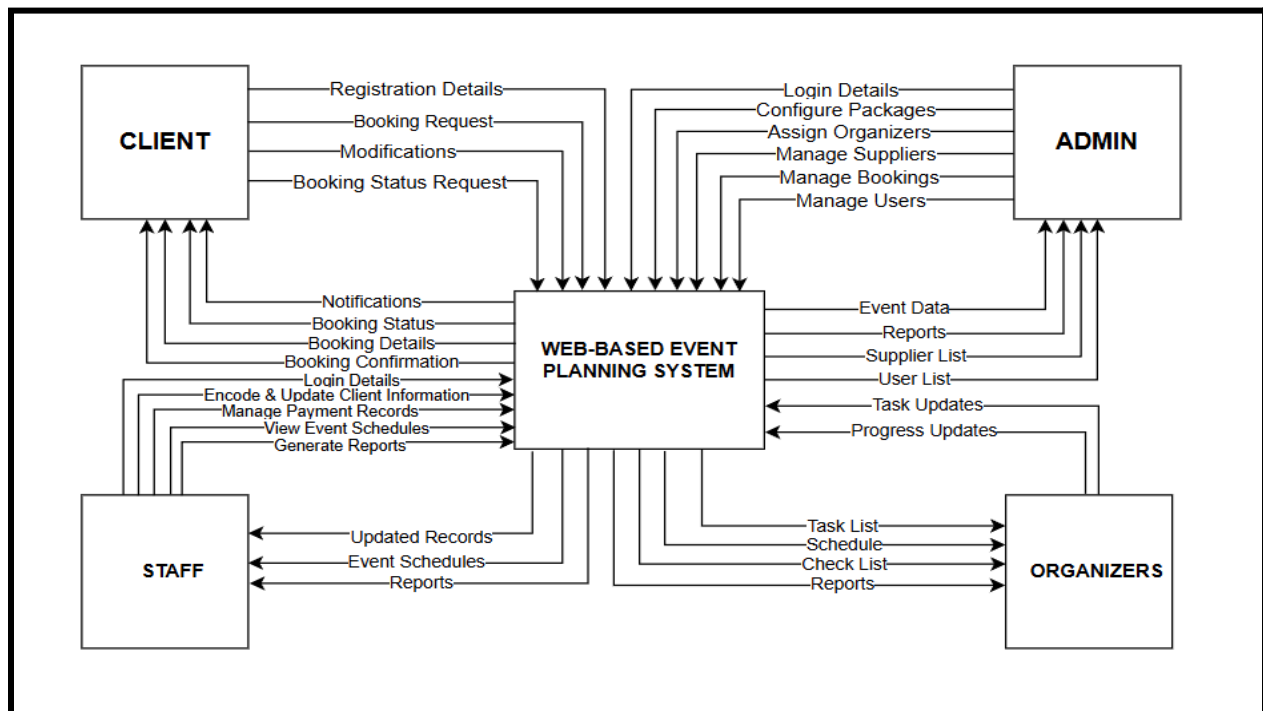
Figure 4.2. Level 0 Context Diagram of the Web-Based Event Planning System with Budget Tracking
