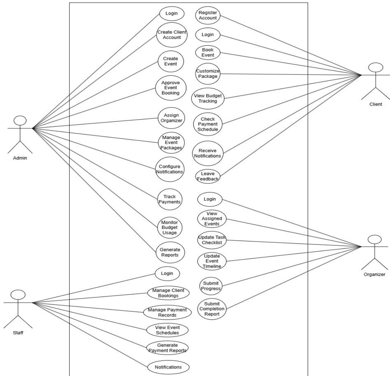
Figure 4.8 - Use Case Diagram
