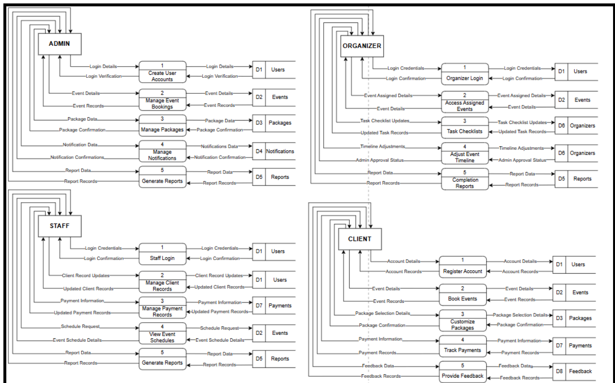
Figure 4.32 Data Flow Diagram
