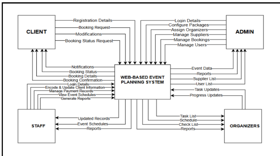
Figure 4.11 : DFD Level 0
