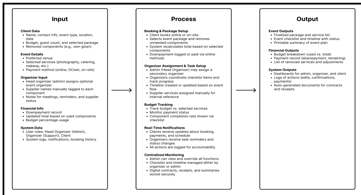
Figure 1.1 Input - Process - Output Model of Web-Based Event Planning System with Budget Tracking
